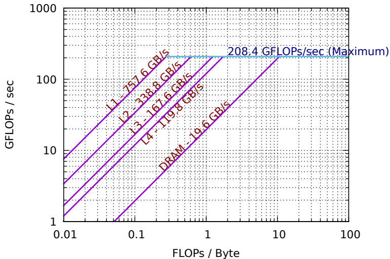
Empirical Roofline Graph (OpenMP/Run.001)
