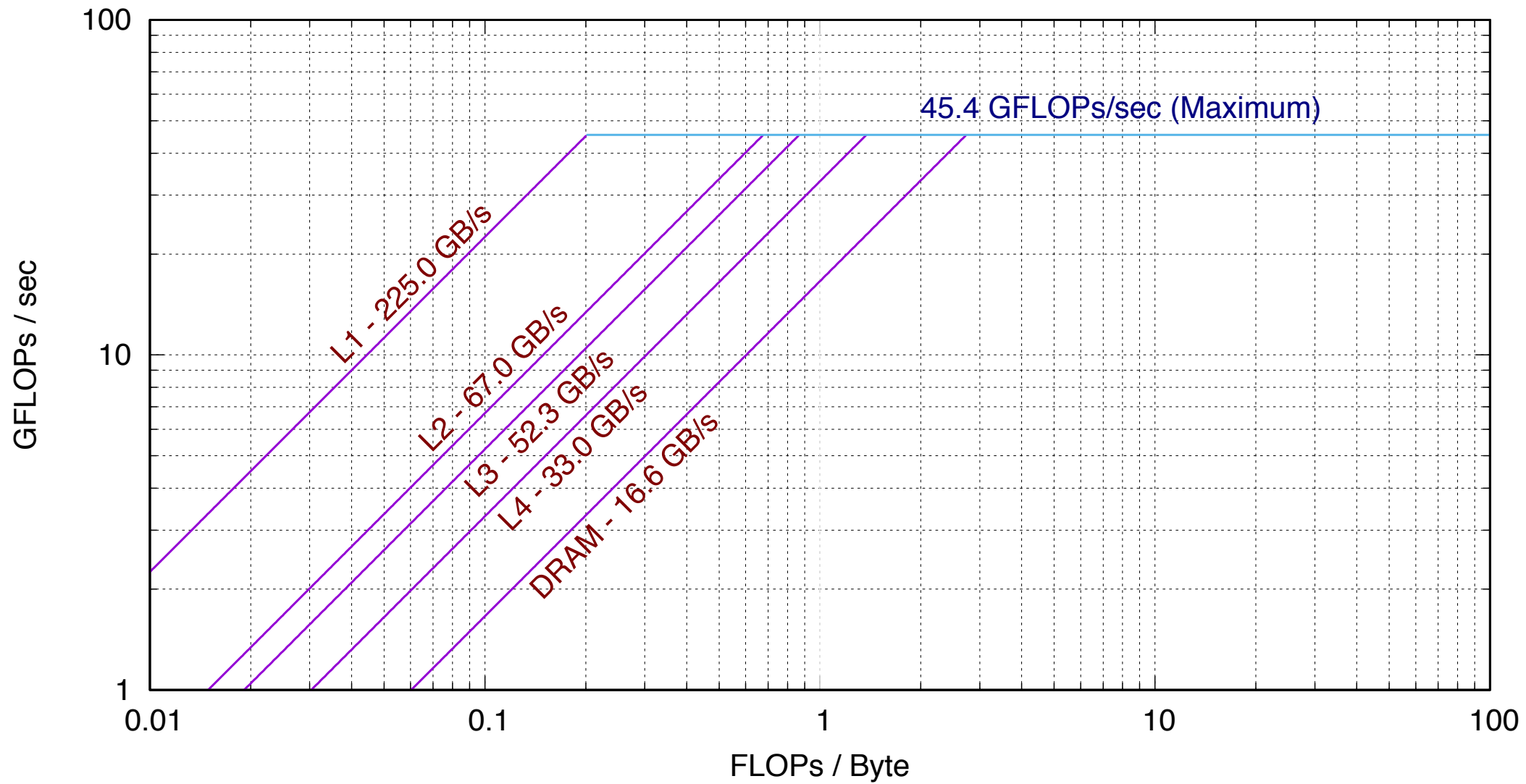
Empirical Roofline Graph (Results.WE31821/Run.004)
